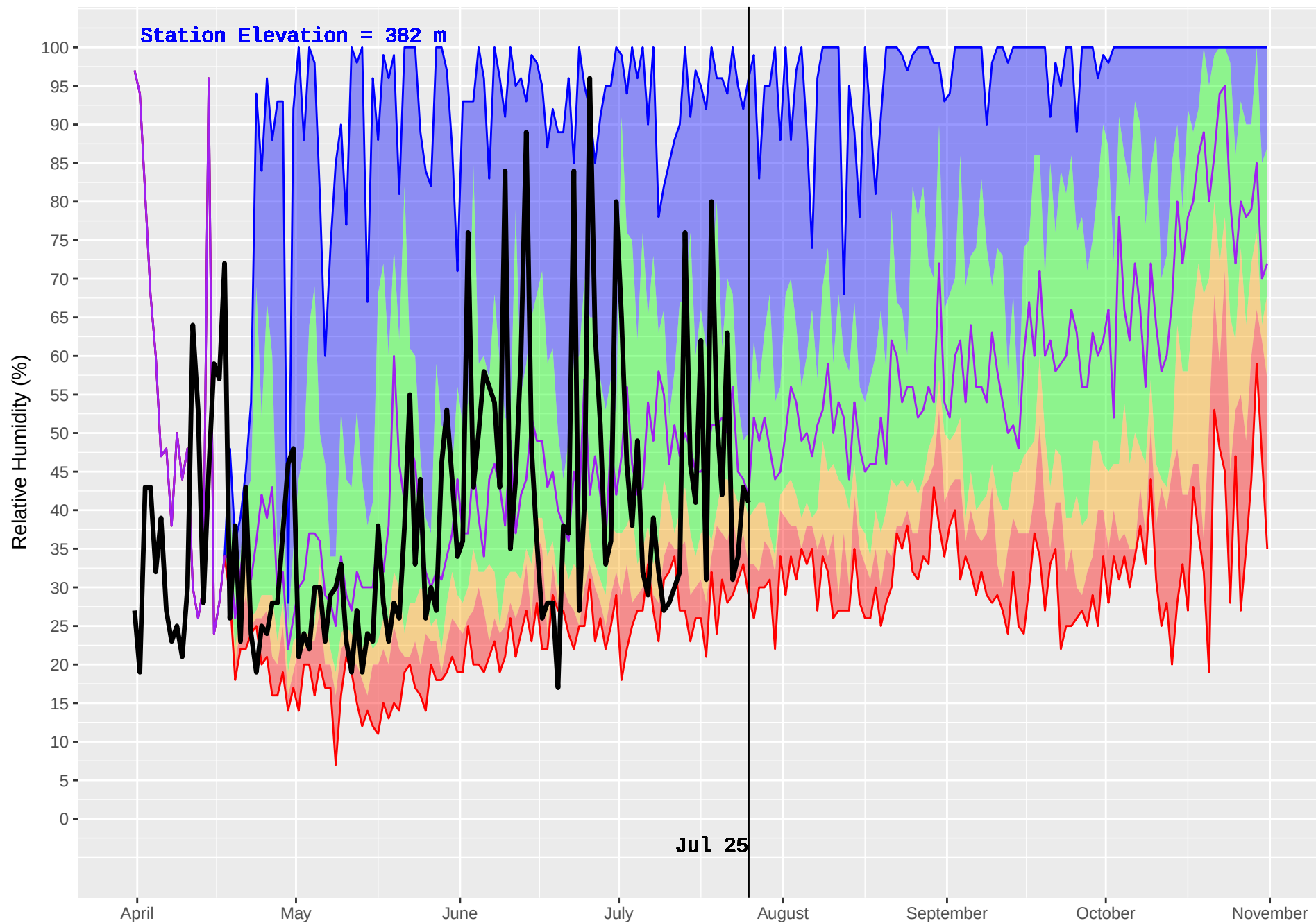
FORT NELSON FS (599) : Historical (1999–2016) and Current (2018) Noon Relative Humidity
