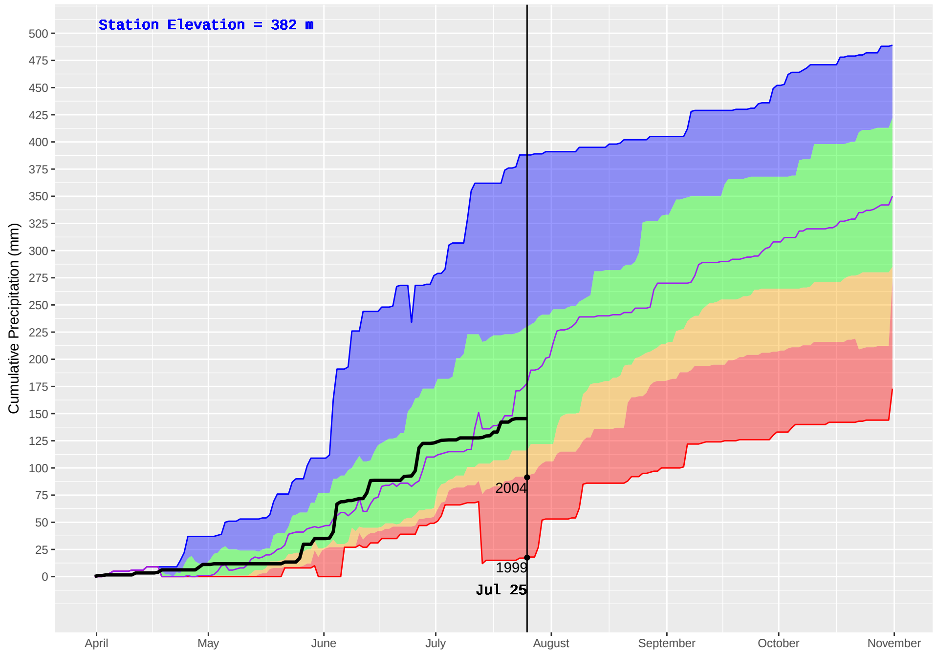
FORT NELSON FS (599) : Historical (1999–2016) and Current (2018) Noon Cumulative Precipitation
