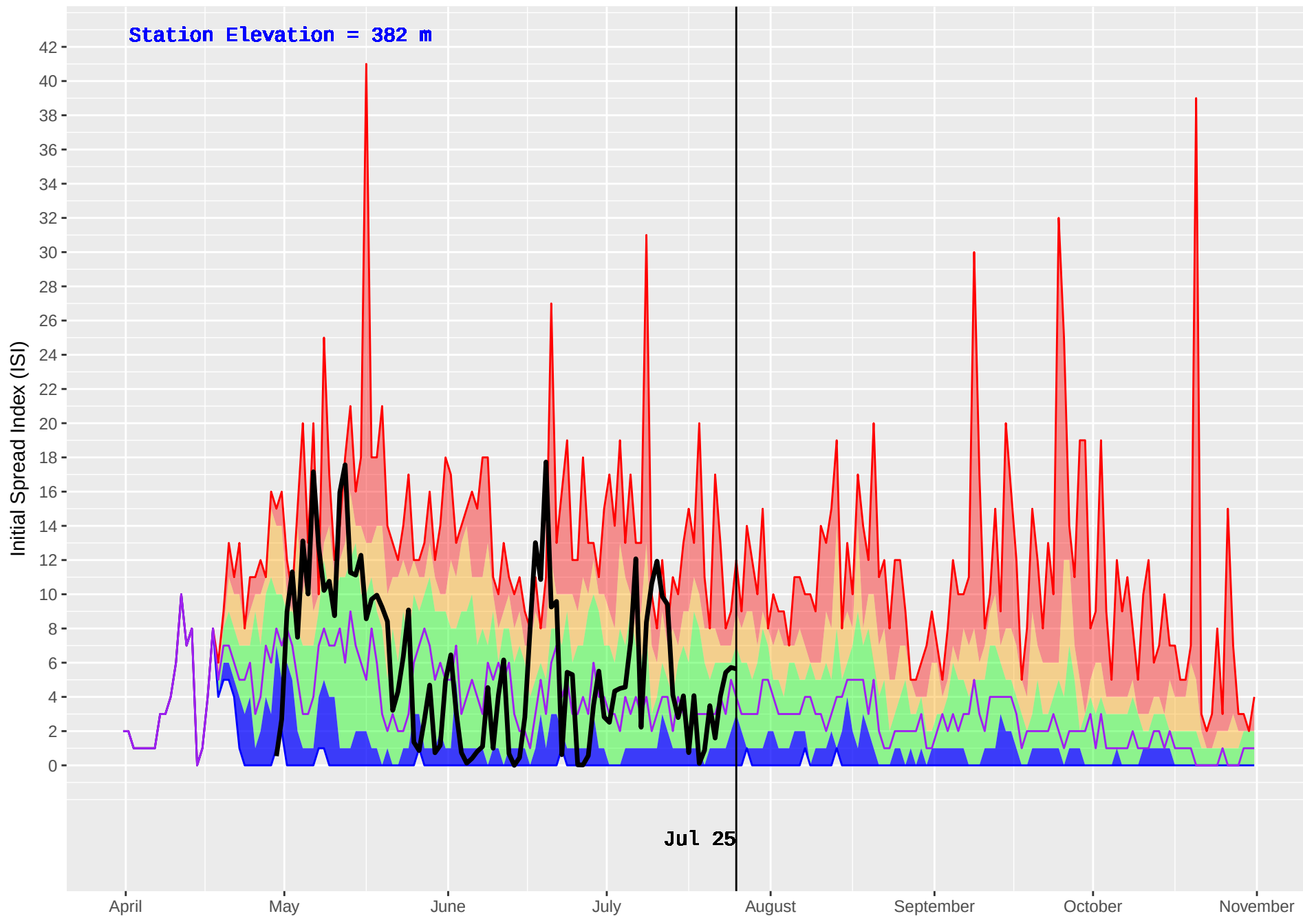
FORT NELSON FS (599) : Historical (1999–2016) and Current (2018) Noon Initial Spread Index (ISI)
