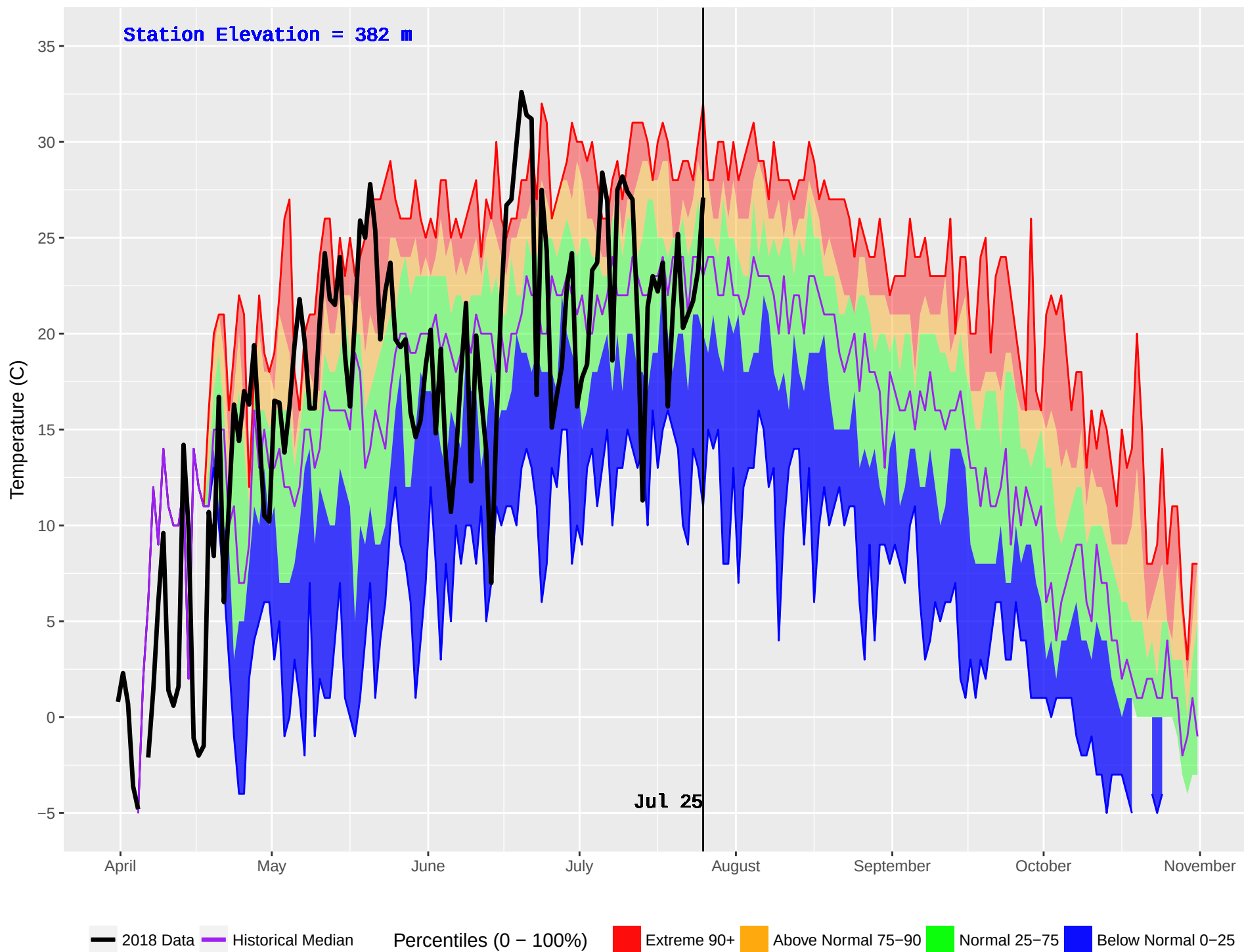
FORT NELSON FS (599) : Historical (1999–2016) and Current (2018) Noon Temperature
