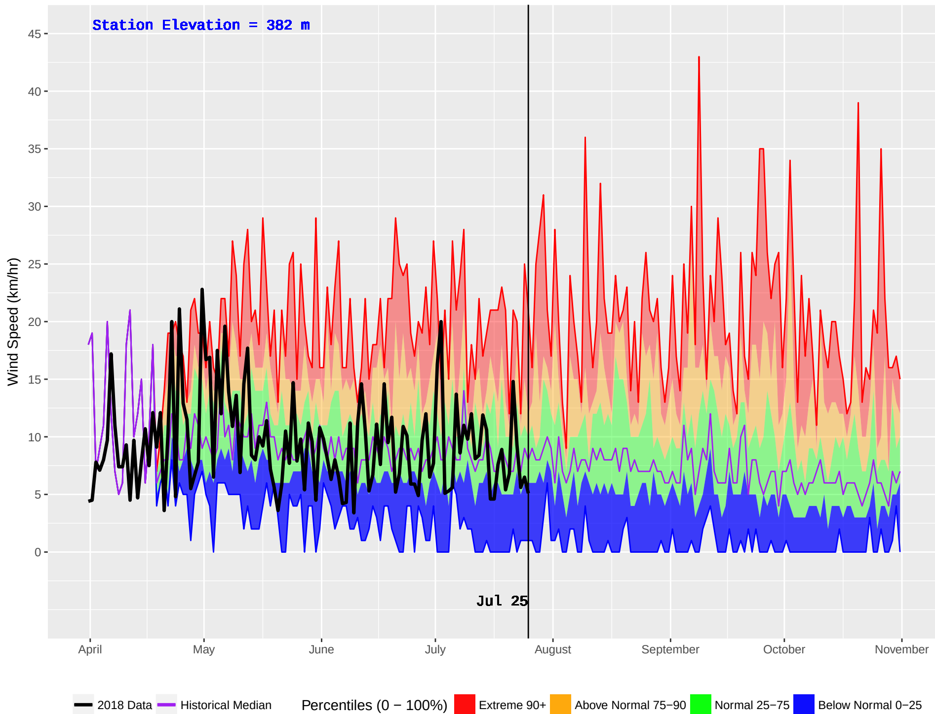
FORT NELSON FS (599) : Historical (1999–2016) and Current (2018) Noon Wind Speed
