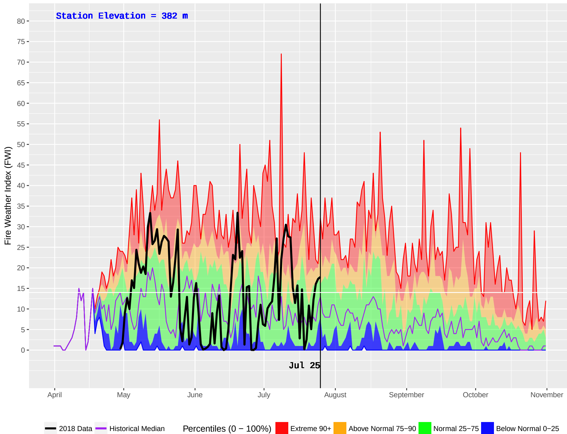
FORT NELSON FS (599) : Historical (1999–2016) and Current (2018) Noon Fire Weather Index (FWI)
