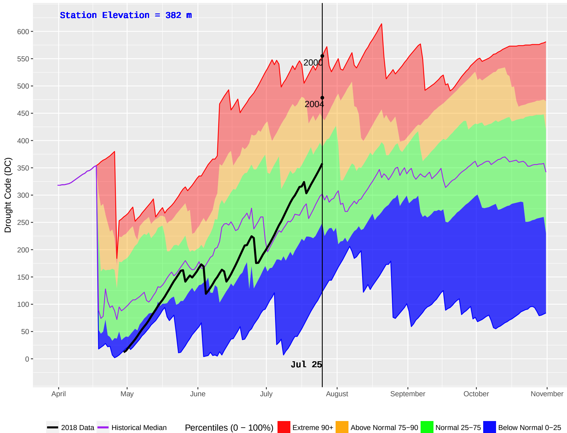
FORT NELSON FS (599) : Historical (1999–2016) and Current (2018) Noon Drought Code (DC)
